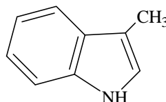
2. Skatole
